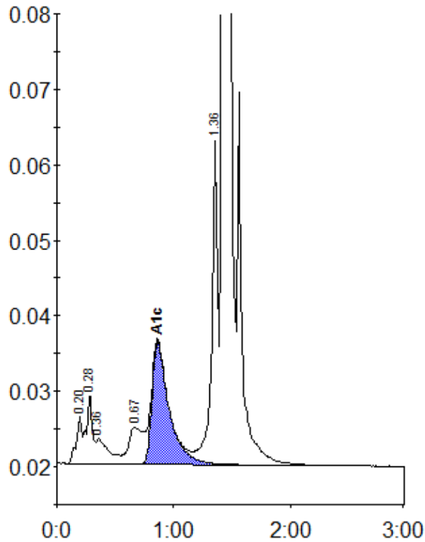
Peak table - ID: 10490771
